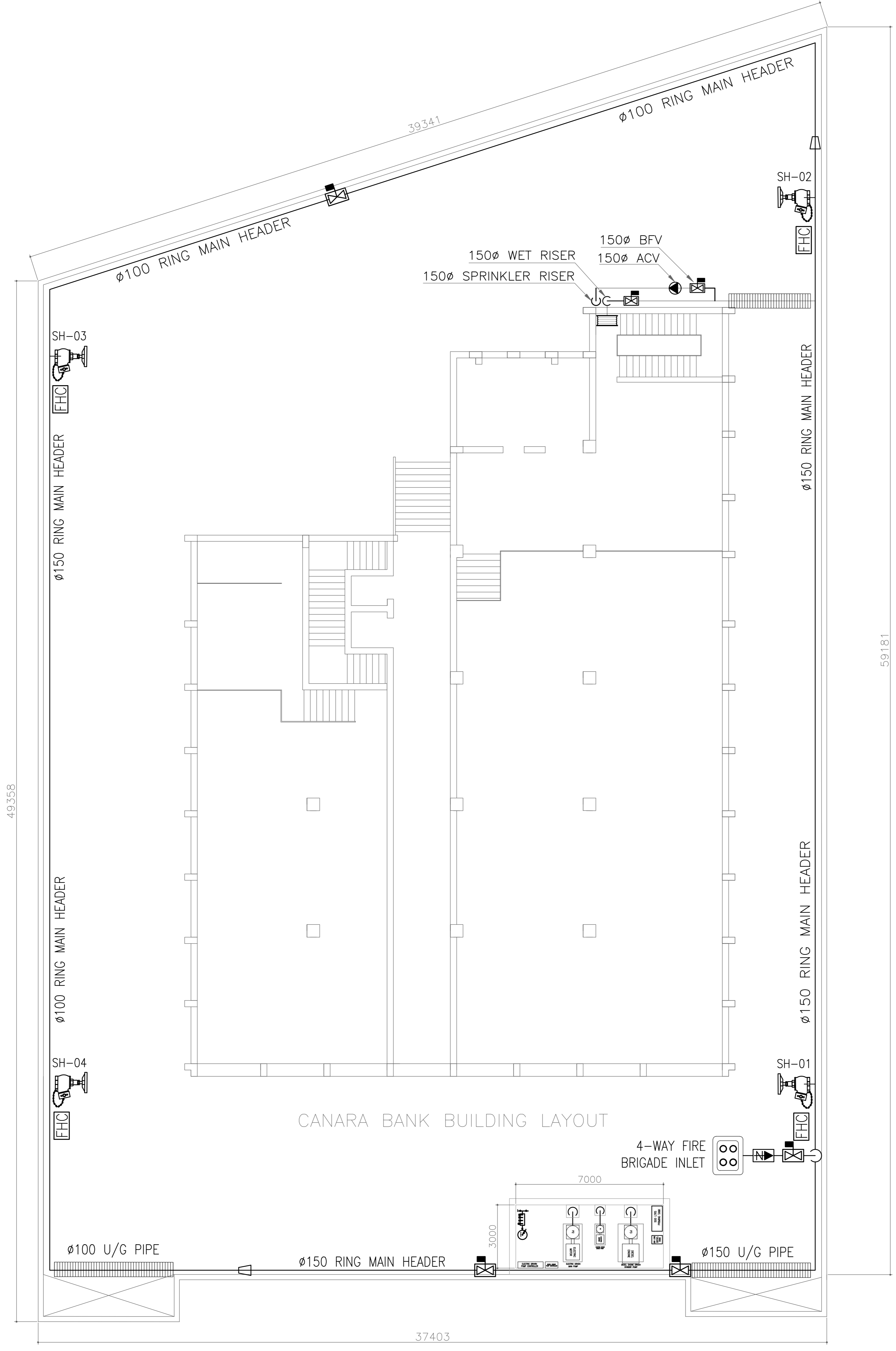
SITE SETTING OUT & EXTERNAL FIRE HYDRANT LAYOUT
