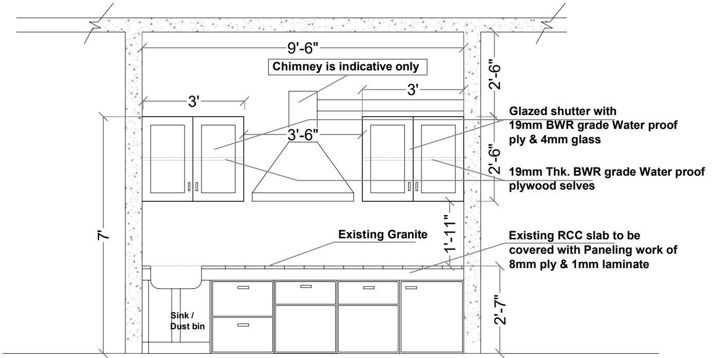
TYPICAL ELEVATION OF KITCHEN
